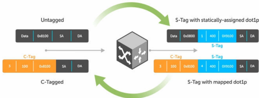
Figure 108. Statically and Dynamically Assigned dot1p for VLAN Stacking
